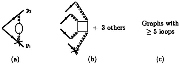
Fig. 10.23. Graphs for the connected part of the derivative of the soft factor, up to four loops. The blob on the gluon line in (a) denotes all corrections to the gluon propagator. The crossed vertex is the same as in Fig. 10.10, and is defined from (10.49). The left-hand ends of the Wilson lines are intended to be joined together, to implement the l.h.s. of (10.100).
