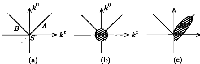
Fig. 10.9. (a) Leading PSSs for one-loop Sudakov form factor. (b) Neighborhood of S for evaluating errors in soft approximation. (c) Neighborhood of A for evaluating errors in collinear-to- A approximation. The squashing on the left indicates that we restrict attention to positive rapidity.
