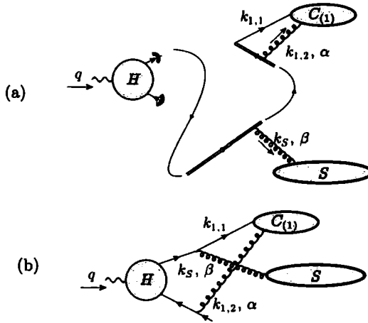
Fig. 12.14. (a) Specific example of Fig. 12.13. Each gluon is labeled with its momentum and color index. (b) A graph that, after approximants and Ward identities are applied, would contribute to (a).
