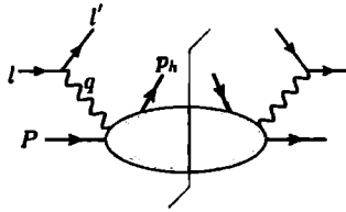
Fig. 12.20. SIDIS cross section.
