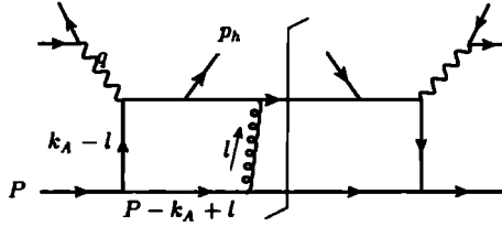
Fig. 12.25. Illustrating Glauber region for (SI)DIS.
