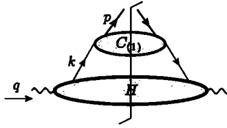
Fig. 12.2. Structure of factorization for one-hadron-inclusive cross section in e^+e^- annihilation.
