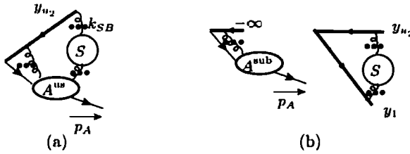
Fig. 10.22. (a) Regions for unsubtracted collinear matrix element (10.90). Here A^{un} is an abbreviation for A^{unsub} . (b) After applying Ward identities to the gluons attaching the soft subgraph to the collinear subgraph, we get this factorized form. Here A^{sub} denotes the subtracted collinear factor. Next to each Wilson line is a label indicating its rapidity.
