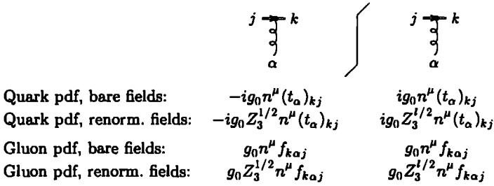
Fig. 7.10. Feynman rules for vertex on Wilson lines in parton densities. Here, n^\mu = \delta_-^\mu = (0, 1, 0_T) . In the Wilson line for a gluon pdf, the generating matrix for the adjoint representation was used: (T_\alpha)_{kj} = if_{k\alpha j} . The sign of the vertex is reversed compared with Collins and Soper (1982b), and corresponds to the sign of the coupling in our Lagrangian, whose Feynman rules are in Fig. 3.1.
