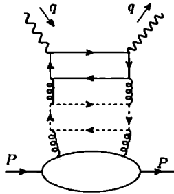
Fig. 11.4. Graph for DIS with Faddeev-Popov ghost loop.
