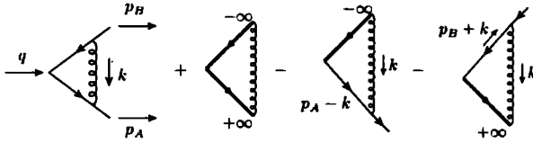
Fig. 10.30. Graphs for one-loop hard coefficient.
