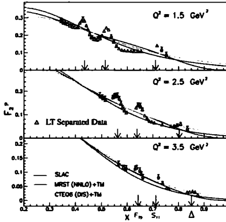
Fig. 11.3. Proton structure function F_2^p measured at Jefferson Lab Hall C. Two of the smooth curves are the results of QCD fits to other data by MRST (Martin et al. , 1998) and CTEQ (Lai et al. , 2000), with target mass corrections included by the method of Barbieri et al. (1976). The SLAC curve is a fit to DIS data (Whitlow et al. , 1992). The arrows indicate the positions of prominent resonances. Reprinted from Melnitchouk, Ent, and Keppel (2005), with permission from Elsevier.
