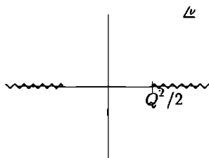
Fig. 5.6. Complex plane in \nu = P \cdot q for T^{\mu\nu} , with its cuts.
