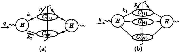
Fig. 12.5. Leading regions in non-gauge theory.
