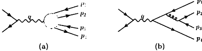
Fig. 4.10. (a) Matrix element of q\bar{q}q\bar{q} fields used to obtain two-pion production. (b) An example of a perturbative graph for the matrix element.
