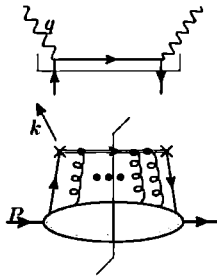
Fig. 7.16. Gauge-invariant form of the parton model.
