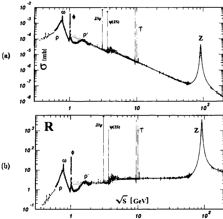
Fig. 4.2. (a) Total cross section and (b) R , for e^+e^- \rightarrow \text{hadrons} . Reprinted from Amstler et al. (2008), with permission from Elsevier. The dashed line is the lowest-order "parton-model" prediction, and the solid line is the 3-loop pQCD prediction from equations (1)–(3) of Chetyrkin, Harlander, and Kuhn (2000).
