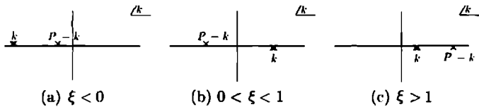
Fig. 6.14. Singularities in k^- plane for (6.121).
