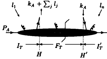
Fig. 14.12. Classification of initial- and final-state interactions. x^+ is assumed to increase from the left to the final-state cut and then decrease again. The soft gluon lines are short to symbolize that their propagators are excluded from the subgraph C_A .
