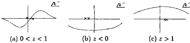
Fig. 5.25. The k^- plane, showing the singularities for the lines k and p_A - k for the three cases 0 < z < 1 , z < 0 , and z > 1 , together with appropriate choices of contour. The scale of the diagram is roughly (k_T^2 + m^2)/p_A^+ ; the pole for the p_B + k line is far off-scale, at k^- = -O(Q^2/p_A^+) .
