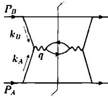
Fig. 5.33. Elementary contribution to Drell-Yan with single spectator.
