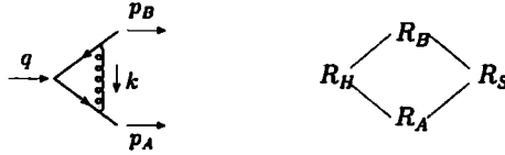
Fig. 10.4. One-loop graph for Sudakov form factor, and the hierarchy of its leading regions. In each case, the name of the region, e.g., “ R_S ”, refers to the category of the gluon’s momentum. A line connecting two regions denotes that they are ordered, with the bigger region on the left. Thus the diagram component R_2 - R_1 means that R_2 > R_1 in the sense defined in Sec. 10.1.2.
