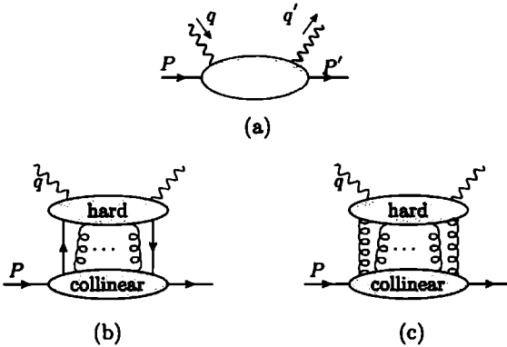
Fig. 11.5. (a) Uncut amplitude for DVCS or DIS. (b) and (c) Leading regions.
