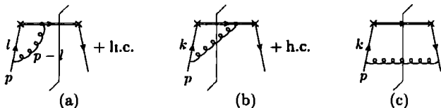
Fig. 9.2. One-loop graphs for renormalization of density of quark in quark. Hermitian conjugates of (a) and (b) should be added. As explained in the text, graphs with a quark self-energy graph need not be considered explicitly, and graphs where the gluon connects the Wilson line to itself are zero.
