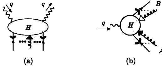
Fig. 11.6. Hard subgraph H with K gluons attached. The thick curved lines indicate where an external quark is set on-shell in H . The triangle indicates the application of a Grammer-Yennie K approximant, defined as in Sec. 10.4.2. Graph (a) is for DIS, with one collinear subgraph. Graph (b) is for e^+e^- annihilation in the simplest case of two collinear groups. Here the solid arrow denotes the approximant for collinear- A gluons and the open arrow denotes the approximant for collinear- B gluons.
