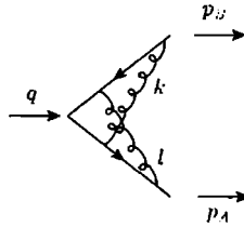
Fig. 5.39. Two-loop vertex graph.
