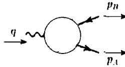
Fig. 5.1. Green function for e^+e^- annihilation to a quark-antiquark pair.
