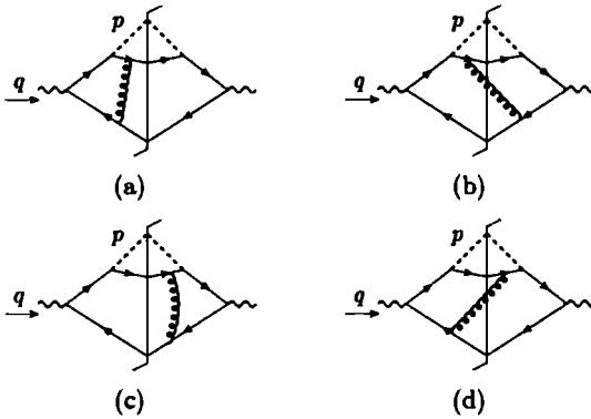
Fig. 12.8. The same as Fig. 12.7, but with soft gluon emission off the external quark in the upper jet.
