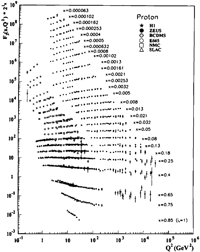
Fig. 2.6. Compilation by the Particle Data Group of data on F_2 on a proton target. For the purpose of separating the different sets of data the values of F_2 have been multiplied by 2^{i_x} , where i_x is the number of the x bin, ranging from i_x = 1 for x = 0.85 to i_x = 28 for x = 0.000063 . Reprinted from Amsler et al. (2008), with permission from Elsevier.
