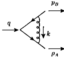
Fig. 5.21. One-loop vertex graph.
