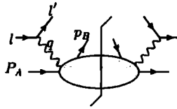
Fig. 13.10. SIDIS cross section.
