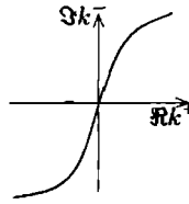
Fig. 7.3. Partially deformed contour for evaluation of integral at zero external p^+ . Note that the axes are the real part of k^+ and the imaginary part of the other variable k^- , and that there are therefore two other dimensions not shown, for \Re k^- and \Im k^+ .
