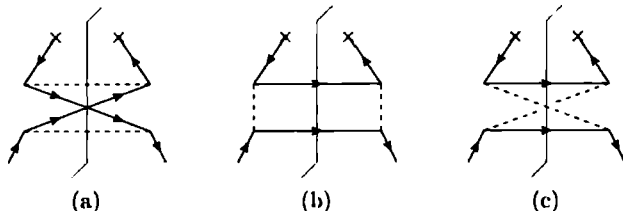
Fig. 8.8. Lowest-order graphs, order g^4 , for evolution of quark to antiquark.
