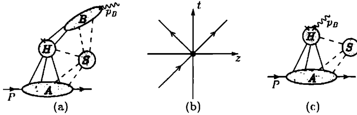
Fig. 5.16. (a) Reduced graphs and (b) space-time diagram, for DVCS and exclusive electroproduction of mesons. (c) Extra reduced graphs for DVCS, but not exclusive meson electroproduction, with photon directly connected to H .
