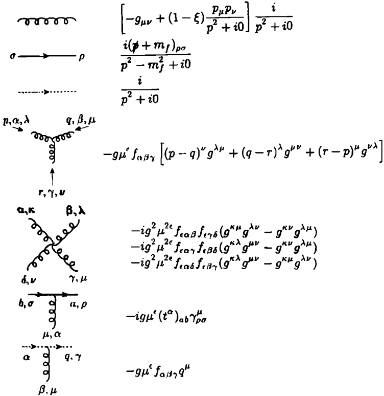
Fig. 3.1. Basic Feynman rules of QCD. The coupling has been replaced by g\mu^\epsilon , according to the standard convention for use in 4 - 2\epsilon dimensions. Propagators and vertices are diagonal in any indices (flavor or color) that are not explicitly indicated. For the renormalization counterterm vertices, see Fig. 3.2.
