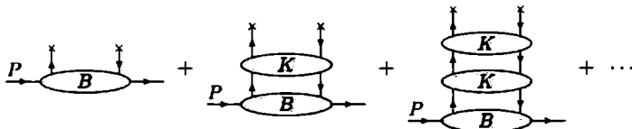
Fig. 8.6. Ladder decomposition of graphs for a bare parton density in terms of two-particle irreducible subgraphs.
