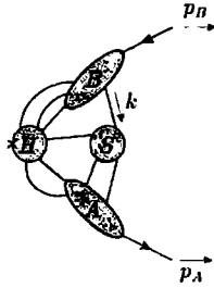
Fig. 5.29. Reduced graph for vertex.
