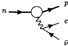
Fig. 2.1. Lowest-order weak interaction for neutron decay.
