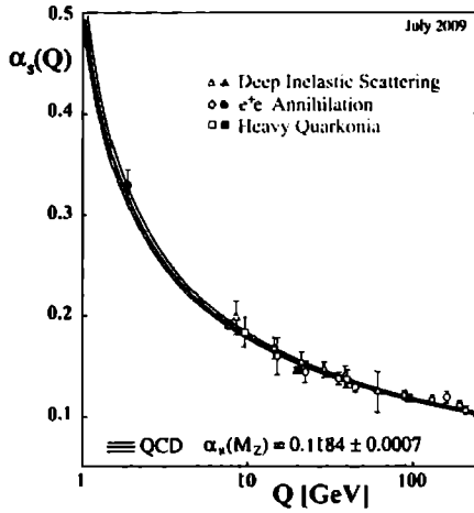
Fig. 3.6. QCD effective coupling. With kind permission from Springer Science+Business Media: Beihke (2009, Fig. 6). The lines represent the solution of the RGE for \alpha_s(\mu) with the \pm\sigma limits on the constant of integration. The scheme used is \overline{\text{MS}} with a variable number of active quarks, as in Sec. 3.10. The data are, in increasing order of \mu , from fits to the \tau width, \Upsilon decays, DIS, e^+e^- event shapes at 22 GeV at JADE, shapes at TRISTAN at 58 GeV, Z width, and e^+e^- event shapes at 91–208 GeV.
