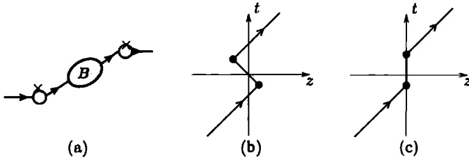
Fig. 11.2. (a) Reduced graph for T^{\mu\nu} at x \simeq 1 . Not indicated are extra collinear lines and a possible soft subgraph. (b) Space-time structure of its massless PSSs when x = 1 . (c) Same with massive intermediate state.
