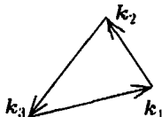
Fig. 4.9. Momentum configuration for 3-body final state.
