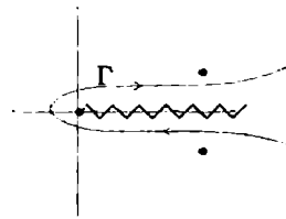
Fig. 4.14. Contour to relate \tilde{R} to \Pi . The off-real-axis singularities are those in the averaging function F(s - Q^2, \Delta^2) . The dots represent the singularities of F .
