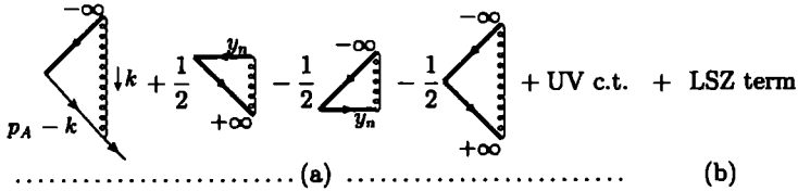
Fig. 10.29. Graphs for A at one-loop, including subtractions and the counterterm for canceling the UV divergence. Next to each double line representing a Wilson line is a label for its rapidity, -\infty , +\infty or y_n . The factors of \frac{1}{2} multiplying the Wilson-line terms arise from the one-loop expansion of the factors in the square root in (10.119a). The upper Wilson lines have the charge of an antiquark . The LSZ term is a self-energy graph for the on-shell quark.
