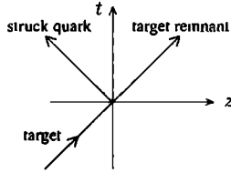
Fig. 6.3. The Libby-Sterman analysis associates these world lines of massless particles in the Breit frame with the leading region that gives the parton model.
