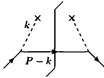
Fig. 6.12. Scalar density in quark.
