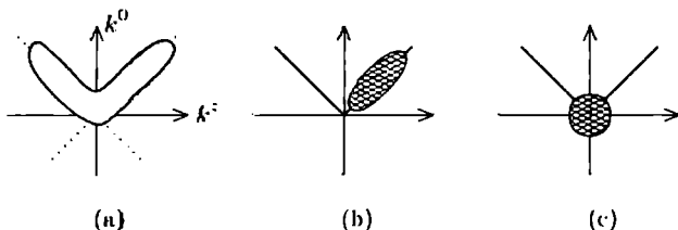
Fig. 5.26. (a) Integration domain used for region H ; it excludes the blanked-out area around the PSSs. The size of the regions shown is a modest factor less than Q . This diagram should be treated as having two more dimensions perpendicular to the ones shown. (b) Integration domain used for region A , the cross-hatched area. (c) Integration domain used for region S .
