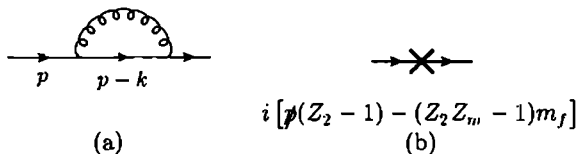
Fig. 3.3. (a) Quark self-energy graph. (b) Counterterm.
