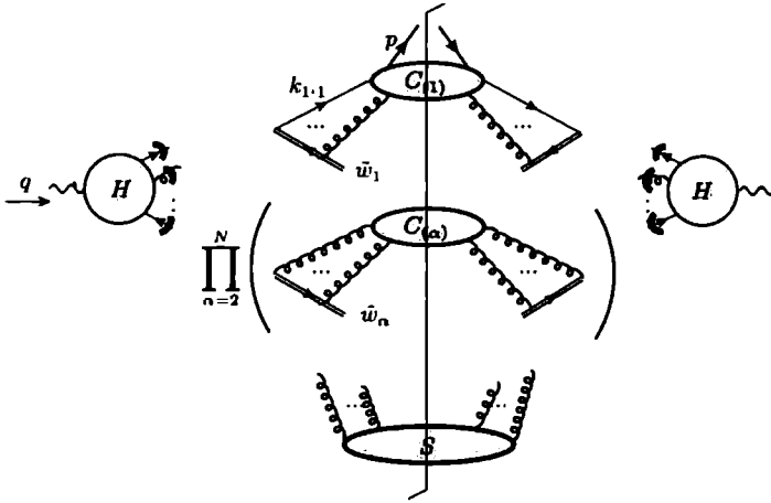
Fig. 12.11. Result of extraction of collinear K gluons from hard subgraphs in Fig. 12.4. There are Wilson lines for each subgraph in the directions shown. The soft subgraph S still couples to the collinear subgraphs. The little thick arcs on the hard subgraphs indicate on-shell partonic lines.
