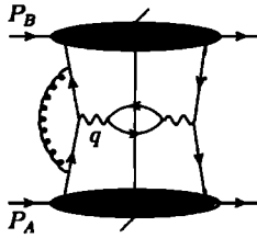
Fig. 14.10. Initial-state interaction of active partons.
