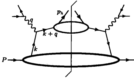
Fig. 12.22. Parton model for SIDIS.
