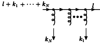
Fig. 7.14. Attachment of collinear gluons to hard quark.
