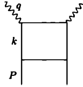
Fig. 10.2. One-loop graph for DIS on elementary target.
