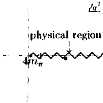
Fig. 4.13. Analyticity in Q^2 for \Pi(Q^2) .
