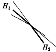
Fig. 12.19. Two-jet configuration with a registered particle (thick lines) in each jet.
