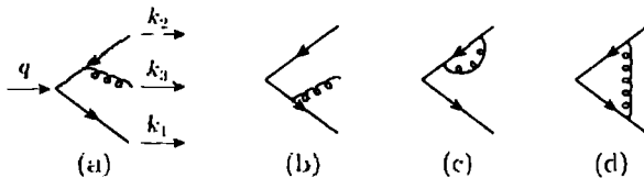
Fig. 4.8. NLO graphs for amplitudes for R .
